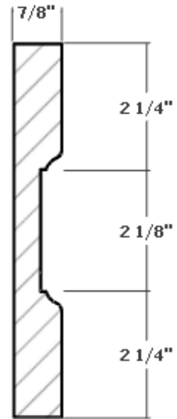
DRAWER DETAIL
